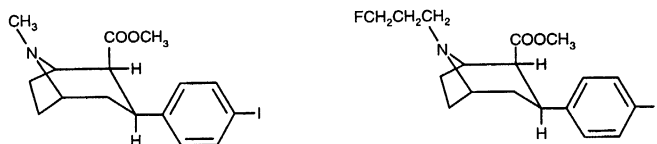
Figure 1. Structures of \beta -CIT (left) and \beta -CFT-FP ( III ) (right)
